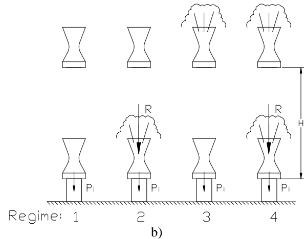
Fig.2. a) Laboratory setup: 1 – hose support roller; 2 – hose for pressure air feed; 3 – falling part; 4 – system for hold up of the falling part in upper position; 5 – tube body; 6 – electronic control unit; 7 – power supply of system 4; 8 – inductive sensors; 9 – base; b) Regimes of the experimental setup: 1 – simple impact; 2 – simple impact + controlled impact; 3 – accelerated by rocket engine simple impact; 4 – accelerated impact + controlled impact; P_i – impact force; R – rocket engine thrust
